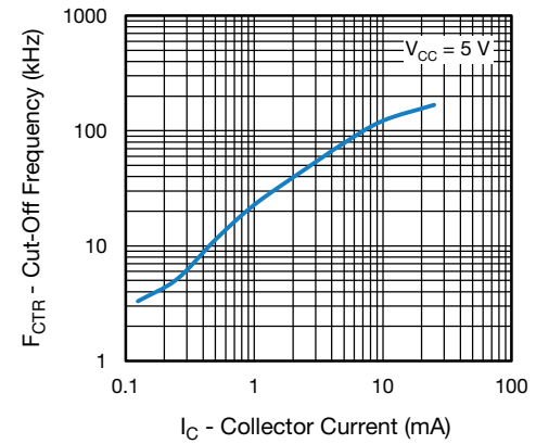
Fig. 15 - Cut-Off Frequency vs. Collector Current
