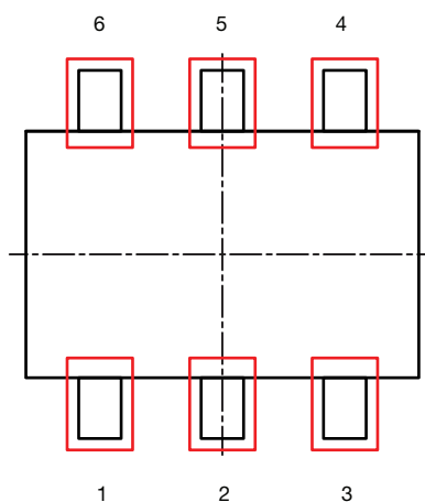
TSOP-6L
