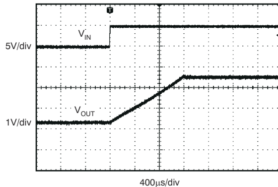
Figure 6-16. Start-Up REF5025, C_L = 10\mu\text{F}
