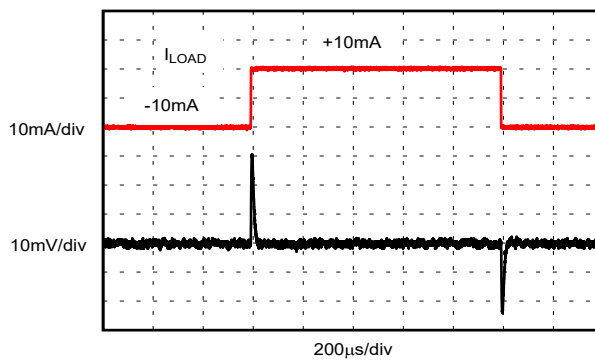
Figure 6-18. Load Transient C_L = 1\mu\text{F} , I_{\text{OUT}} = 10\text{mA}
