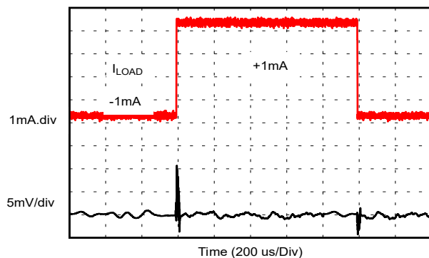
Figure 6-17. Load Transient C_L = 1\mu\text{F} , I_{\text{OUT}} = 1\text{mA}
