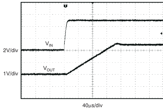
Figure 6-15. Start-Up REF5025, C_L = 1\mu\text{F}
