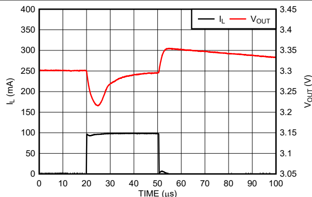
Figure 5-28. Load Transient Response (Legacy Chip)
