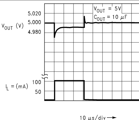
Figure 5-27. Load Transient Response (Legacy Chip)
