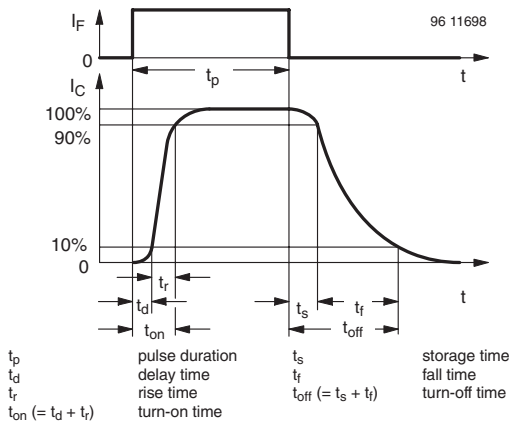
Figure 3. Switching Times
